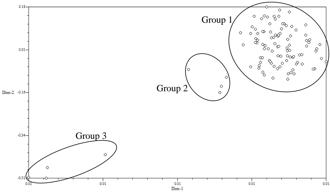
Figure 4. Principle Coordinate Analysis of 105 sea oats lines based on the Dice similarity coefficient.
