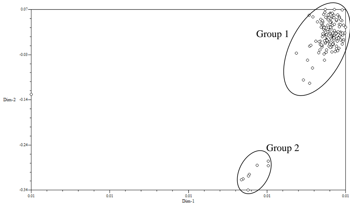
Figure 3. Principle Coordinate Analysis of 156 sea oats lines based on the Dice similarity coefficient.
